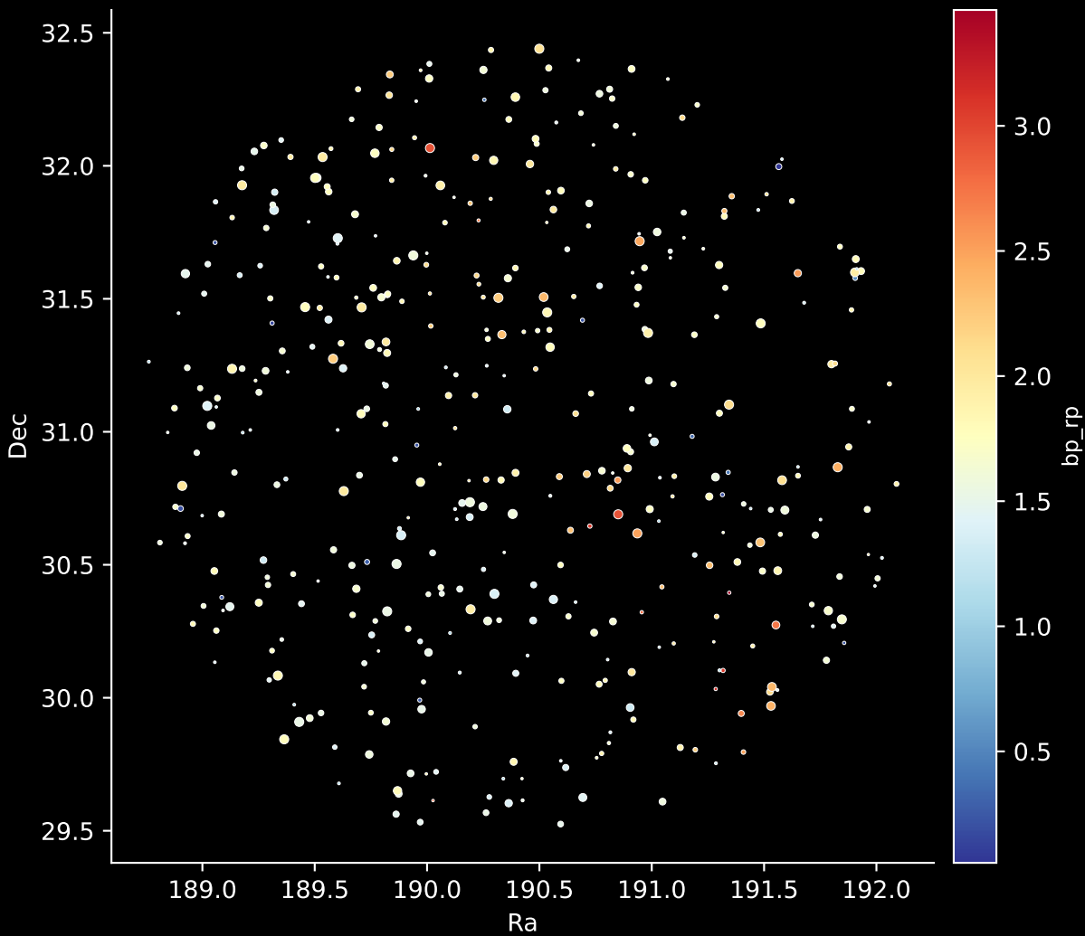
APOGEE DR17 Field: [180+04] Stars: 431
