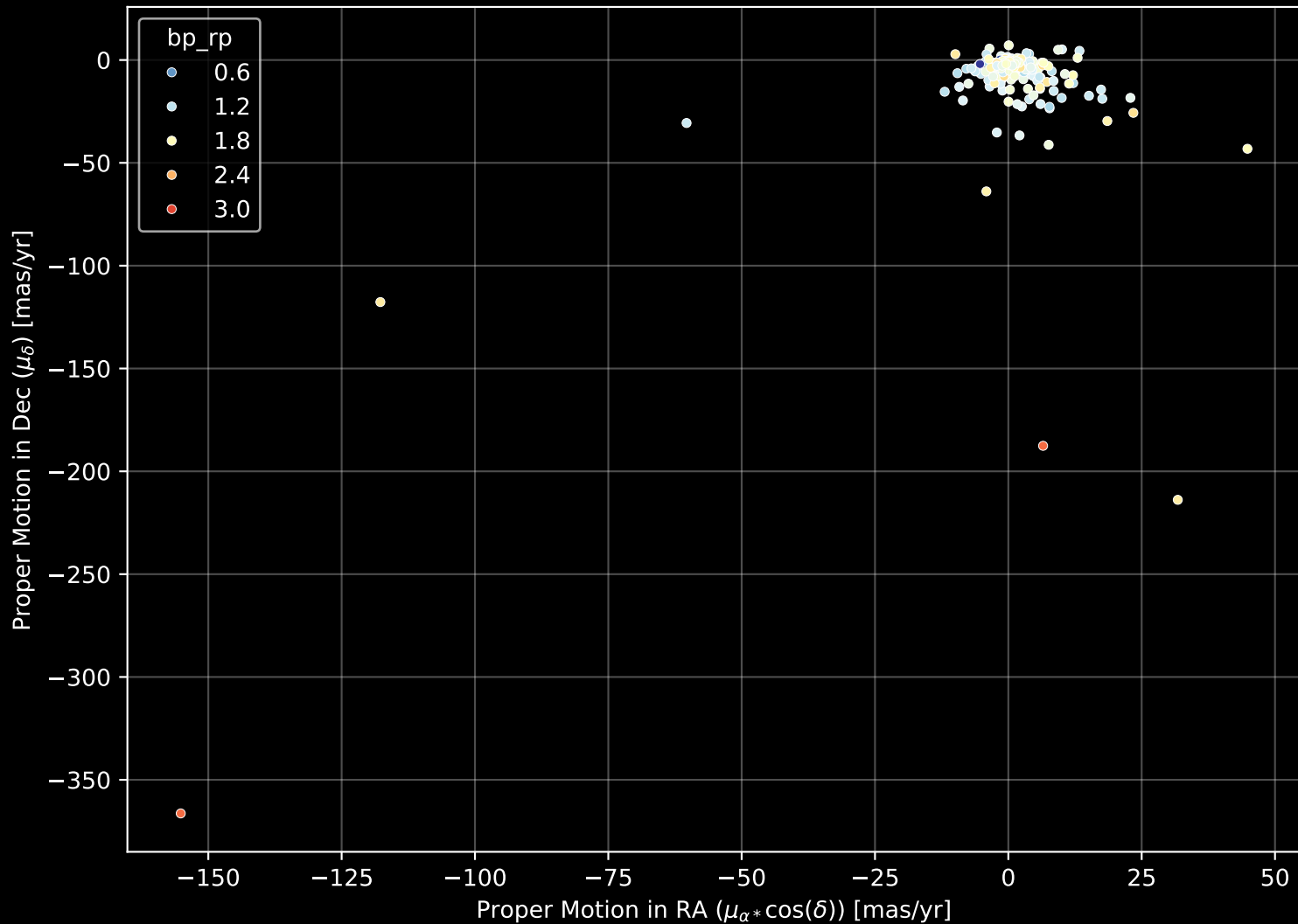
APOGEE DR17 Field: [180+04] Proper Motion Diagram (n= 431)
