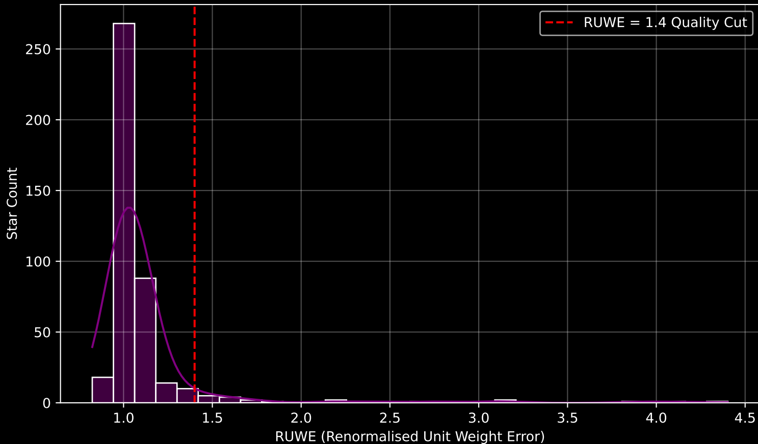
GAPOGEE DR17 Field [180+04] RUWE Distribution (n= 423)
