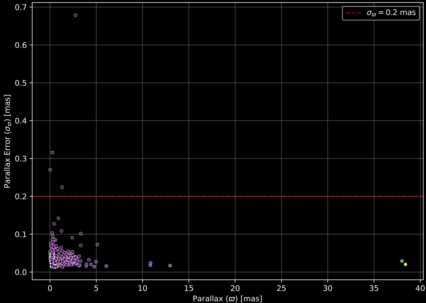
APOGEE DR17 Field: [180+04] Parallax Quality (n= 431)
