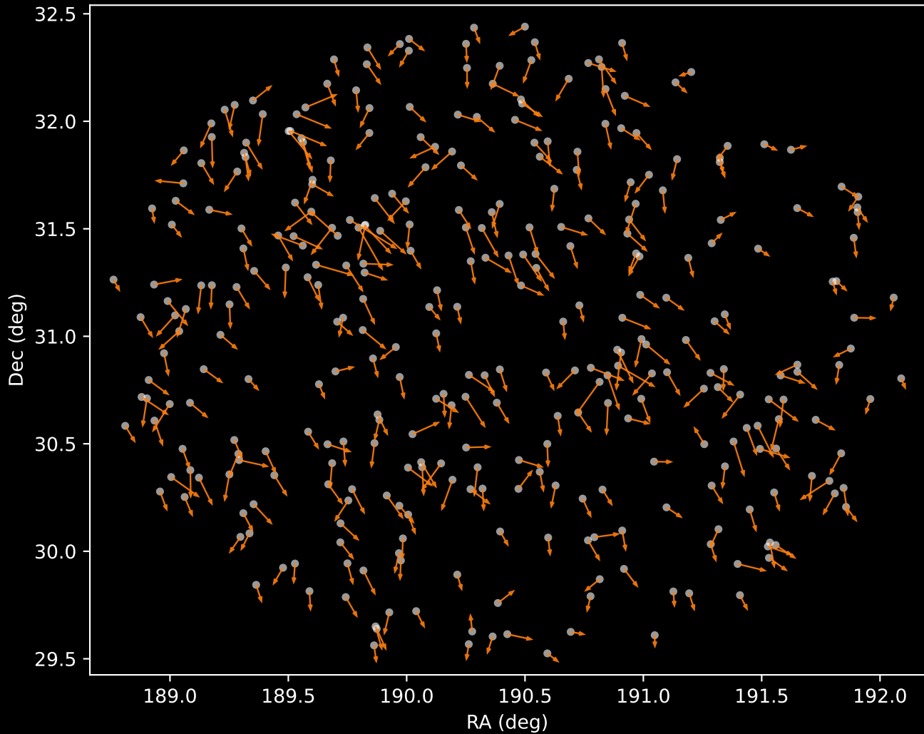
APOGEE DR17 Cluster 2 Proper Motion Vectors (n=336)
