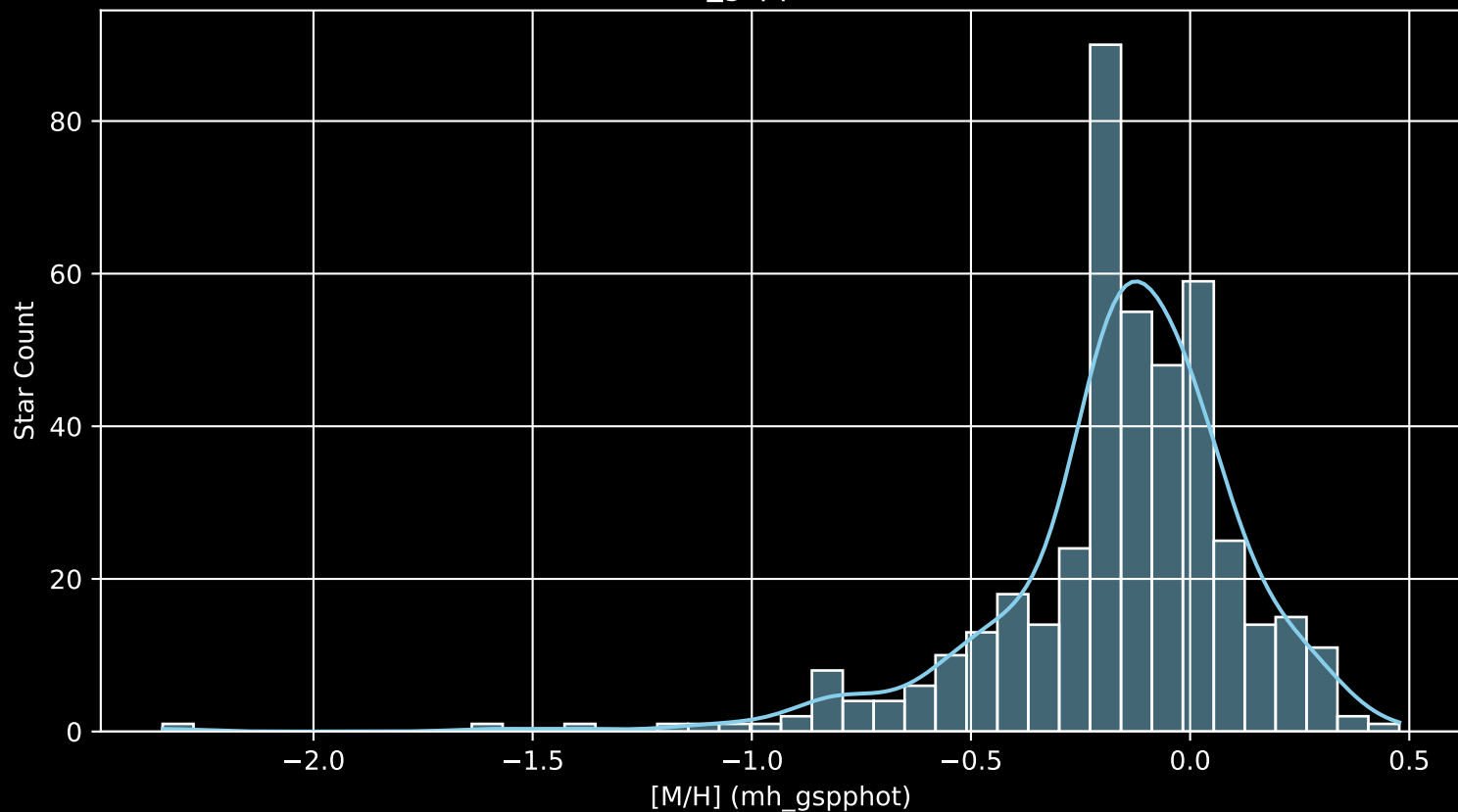
APOGEE DR17 Field: [180+04 [M/H] (mh_gspphot) (n= 430)
